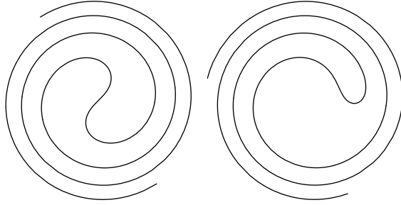
Figure 2: yin-yang curves
