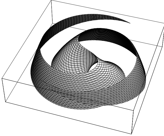
Figure 9: Two-dimensional rotating soliton
