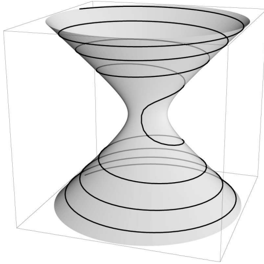
Figure 7: Rotating soliton on a hyperboloid
