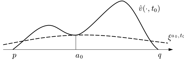
Figure 12: Non-convex set S_{t_0}
