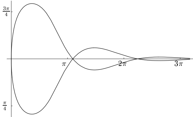
Figure 5: Solution s \mapsto \begin{pmatrix} \varphi(s) \\ r(s) \end{pmatrix}
