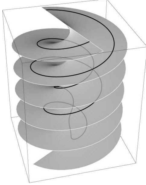
Figure 8: Screwing soliton on a helicoid
