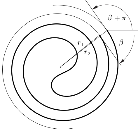
Figure 4: Asymptotic behavior
