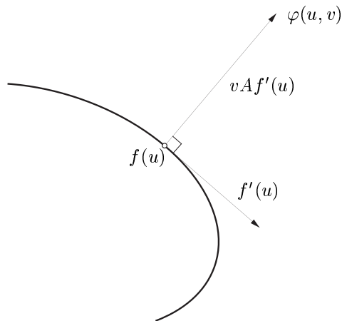
Figure 11: Rotating coordinate system
