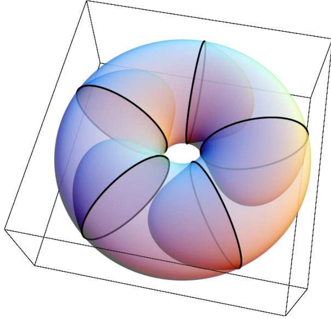
Figure 10: Rotating soliton in a torus
