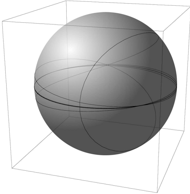
Figure 6: Rotating soliton on a sphere
