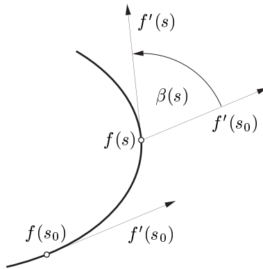
Figure 3: Geometric interpretation
